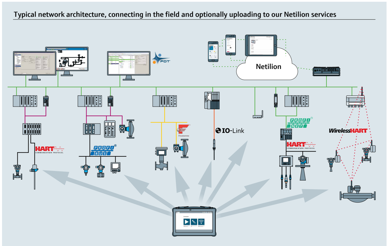
Field Xpert SMT70 communicating with HART, PROFIBUS, FOUNDATION Fieldbus, WirelessHART field devices and more.
